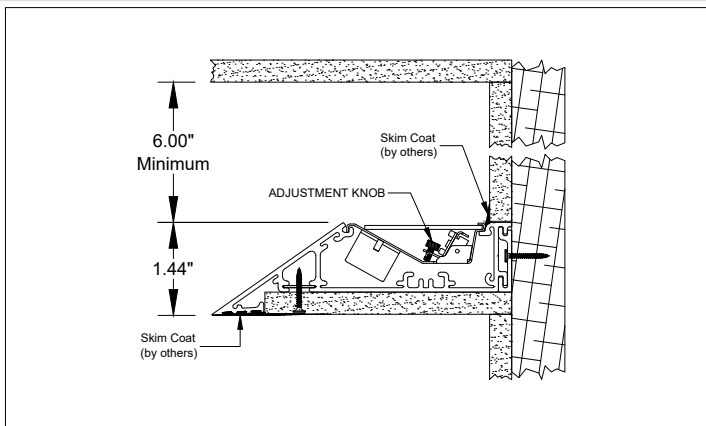
Figure 5. Beam angle adjustment and final installation.
