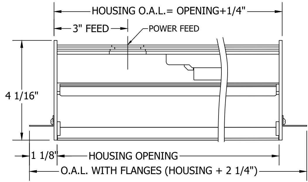
SIDE SECTION
