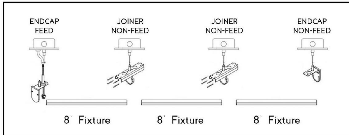
Typical Parts For a 24 Foot Run
